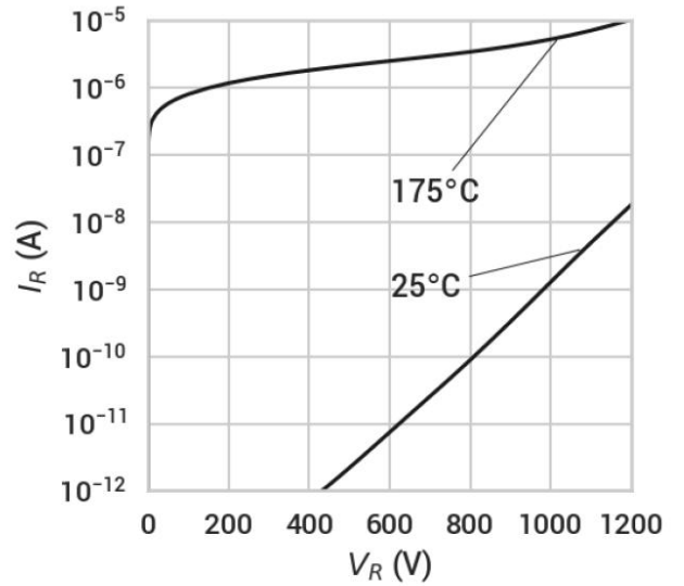
Fig 2. Reverse Characteristics
